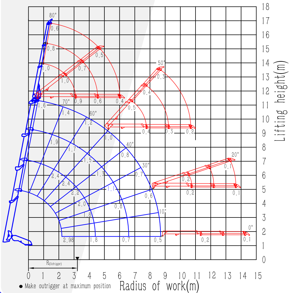
S7 Load Chart With Fly Jib
